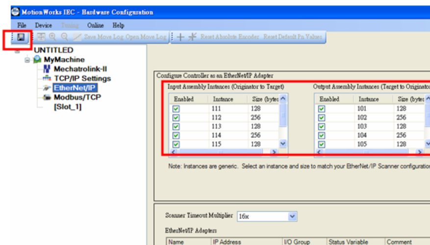
Fig. 1 Assembly Instances
